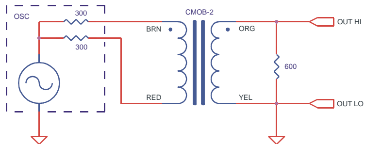
TEST CIRCUIT 4
